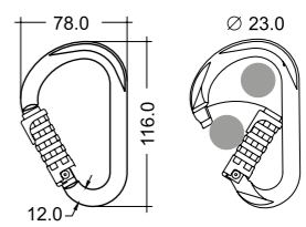
TWIST LOCK #786MG0NNKK
