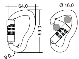
AUTO BLOCK #783IM0NNKK
