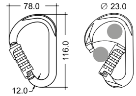
AUTO BLOCK #786MM0NNKK
