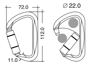
TWIST LOCK #737LG0PNKK
